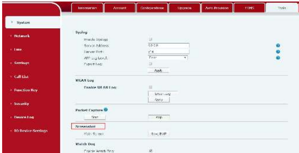
Picture 24- Screenshot
